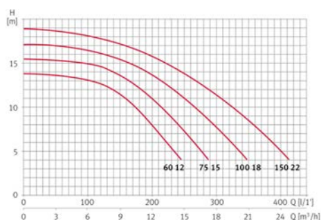
Rendementscurve
